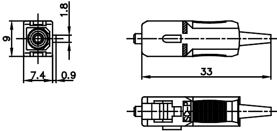
SC Connector for 250um/900um fiber
