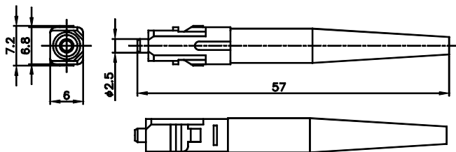
SC2 Connector for 1.6mm/2mm cord
