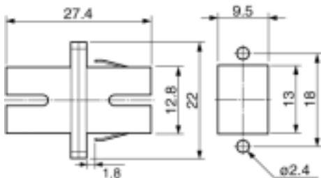
SC-SC Adapter
