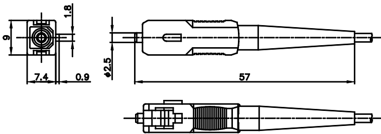
SC Connector for 1.6mm/2.0mm
