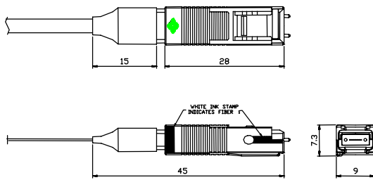
Sumitomo's LIGHTRAY MPX™ for Fiber Ribbon
